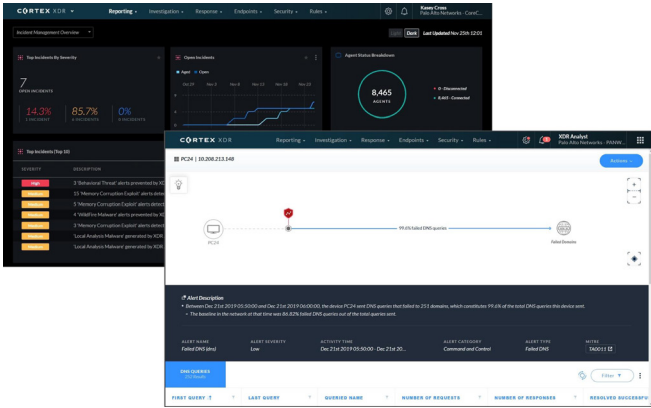
Figure 1: Machine learning and analytics automatically find active threats
