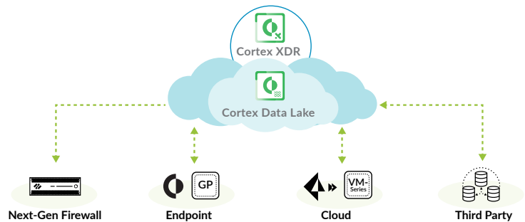
Figure 2: Cortex XDR collects data from Next-Generation Firewalls and third-party sources for network traffic analysis
